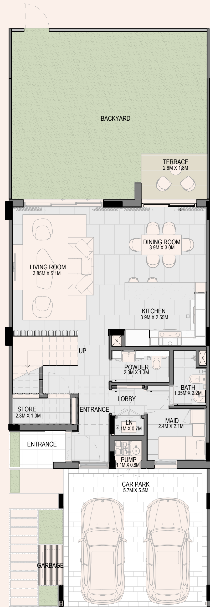
Ground floor
