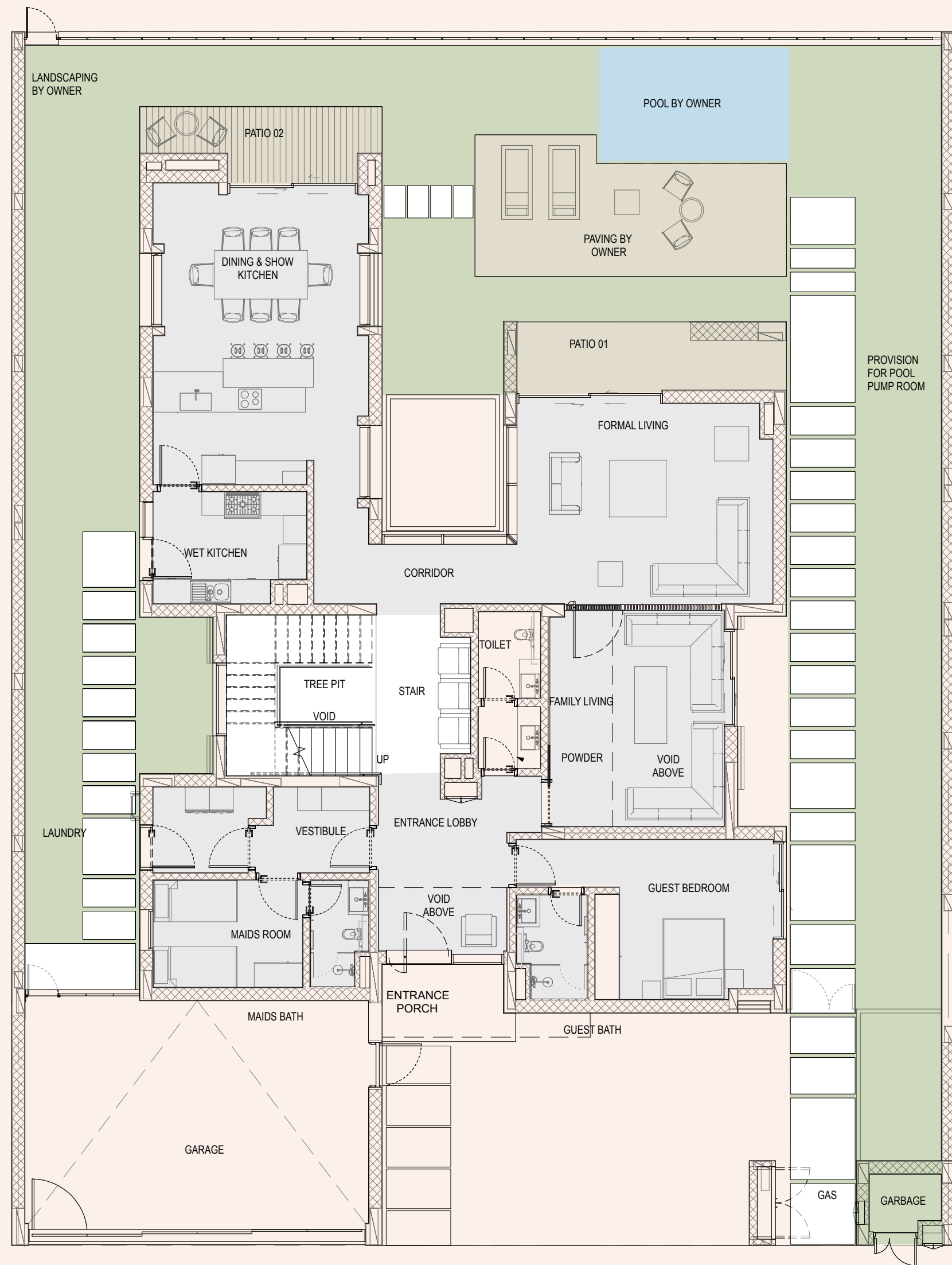
Ground floor
