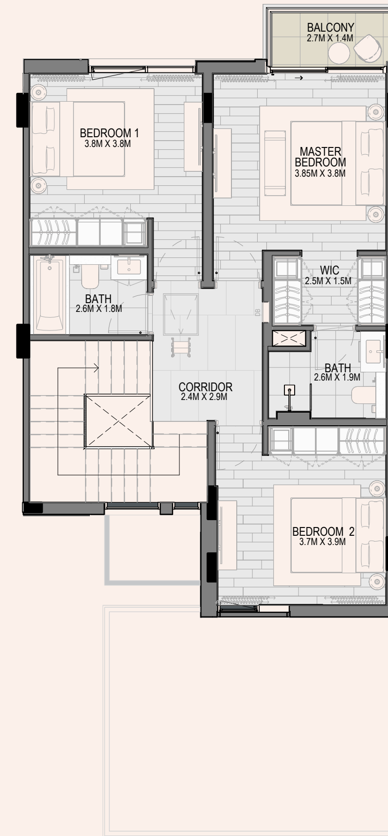
First floor
