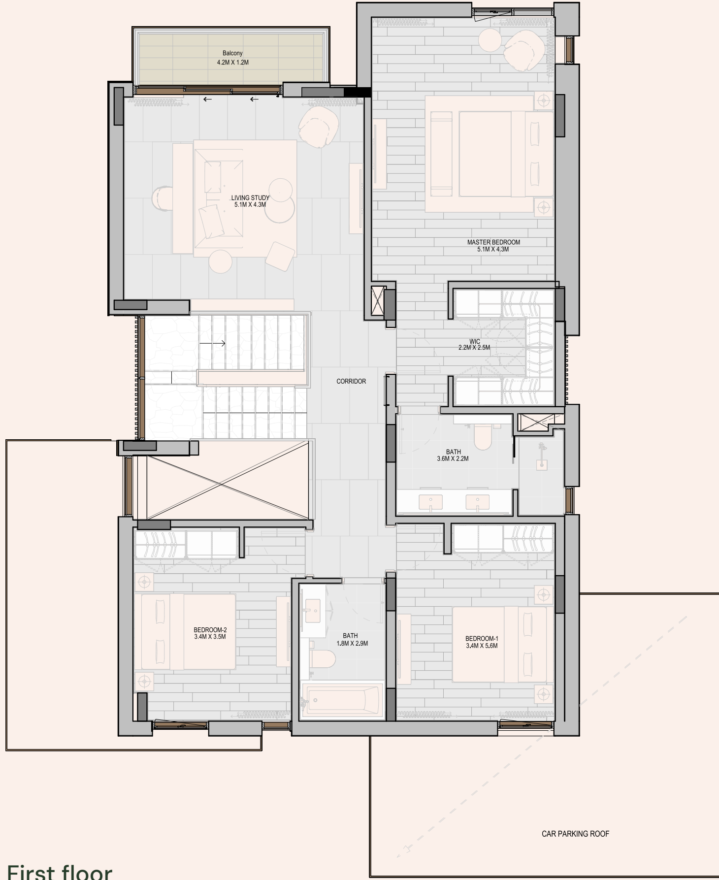
First floor
